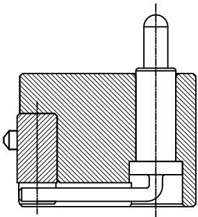
Section A
